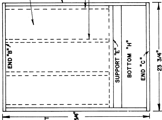
TOP VIEW OF BOX
