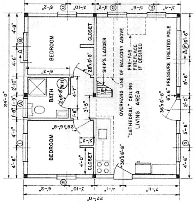
PLAN 0 2 4 6 FT.
